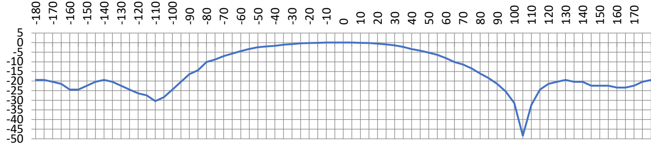
920Mhz Yagi, vertical polarity
